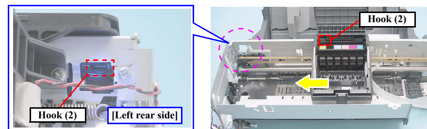
Figure 4-99. Removing the CSIC Assy (2)
