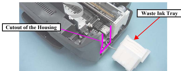
Figure 4-29. Handling of the Waste Ink Tray
