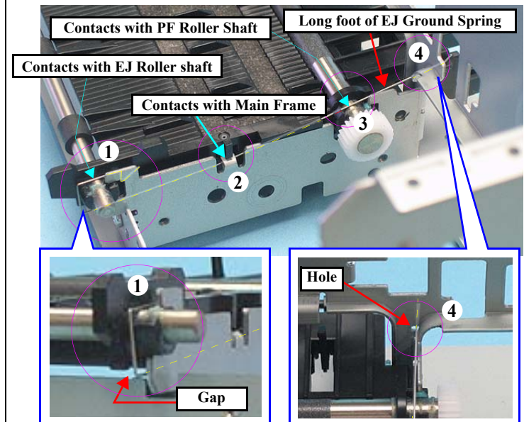
Figure 4-162. Attaching the EJ Ground Spring
