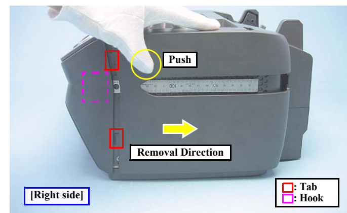
Figure 4-17. Removing the Right/Left Housings (2)
