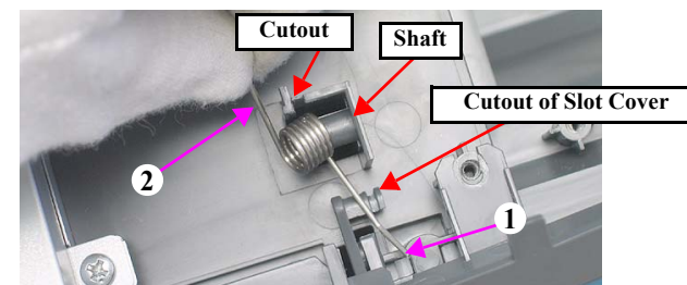
Figure 4-43. Reinstalling the Torsion Spring (R360/R380/R390 only)
