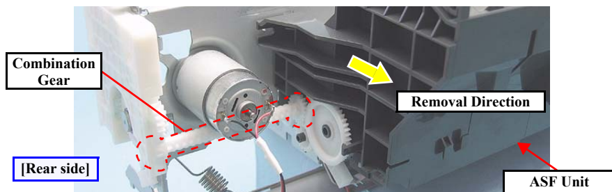
Figure 4-143. Removing the ASF Unit
