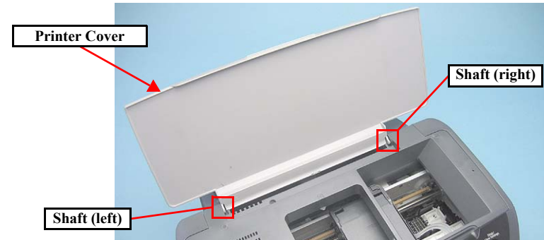
Figure 4-13. Removing the Printer Cover (1)
