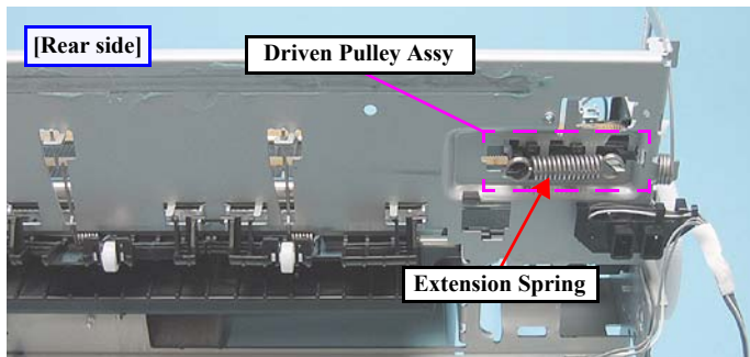
Figure 4-121. Removing the Extension Spring
