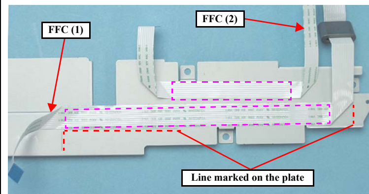
Figure 4-78. Attaching the FFC (1), FFC (2) (R360/R380/R390)
