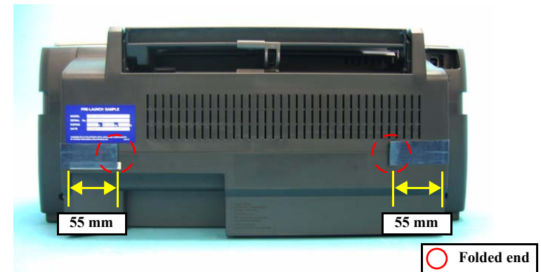
Figure 4-3. Securing the Middle Housing on its rear
