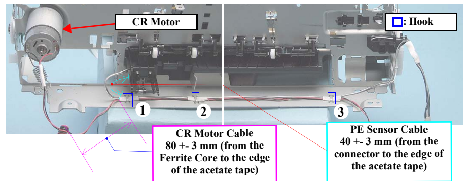
Figure 4-123. Removing the CR Motor (2)
