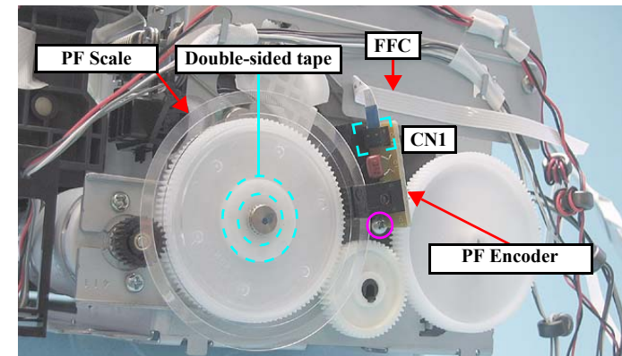
Figure 4-135. Removing the PF Encoder/PF Scale
