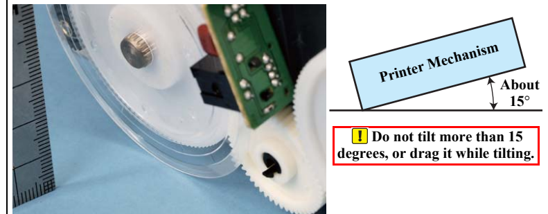
Figure 4-84. Handling of the Printer Mechanism
