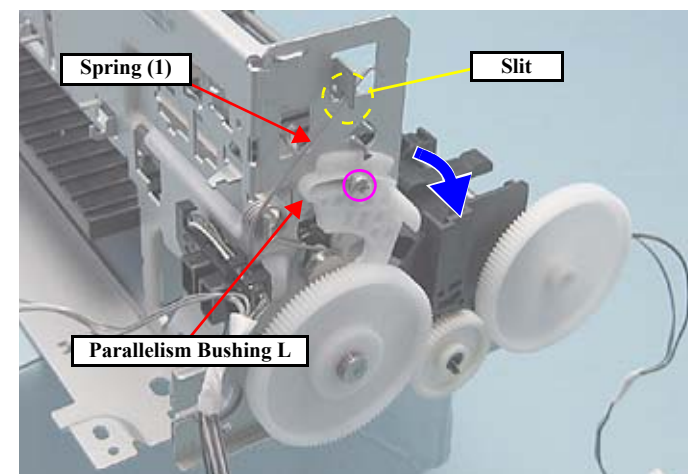
Figure 4-145. Removing the CR Unit (1)
