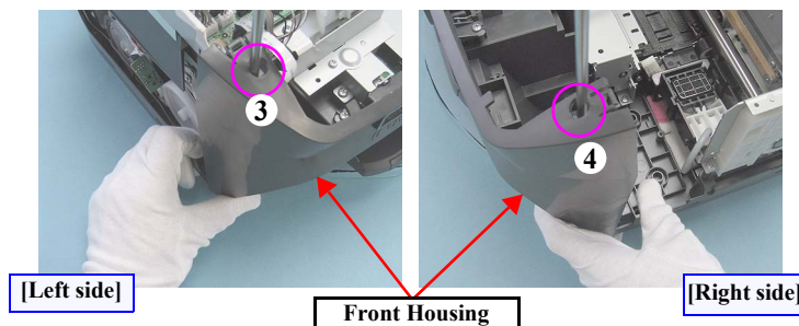
Figure 4-42. Reinstalling the Front Housing (3)
