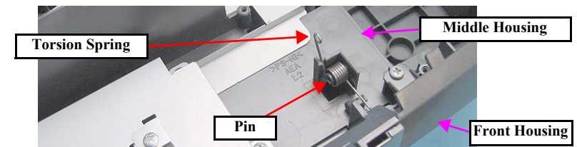
Figure 4-35. Removing the Torsion Spring (R360/R380/R390 only)
