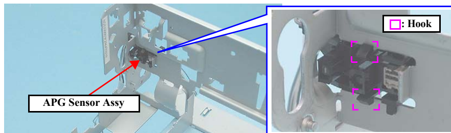
Figure 4-160. Removing the APG Sensor
