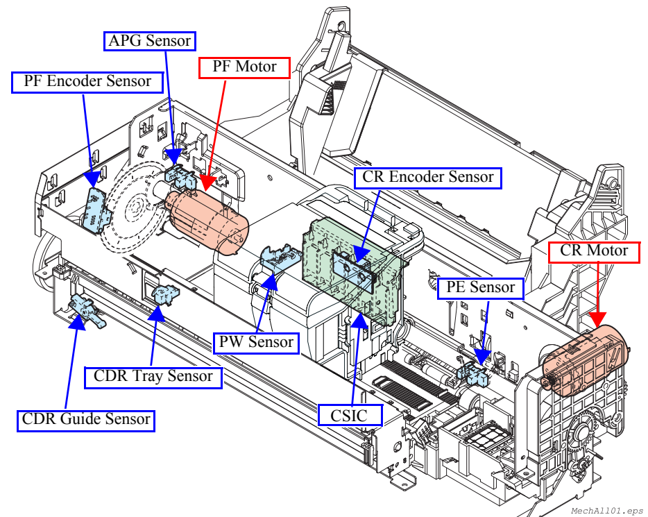
Figure 2-2. Motors & Sensors in the Printer Mechanism
