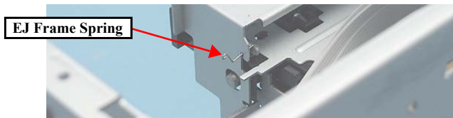
Figure 4-28. Cautions on removing the Waste Ink Tray
