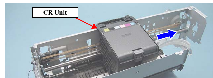
Figure 4-126. Moving the CR Unit
