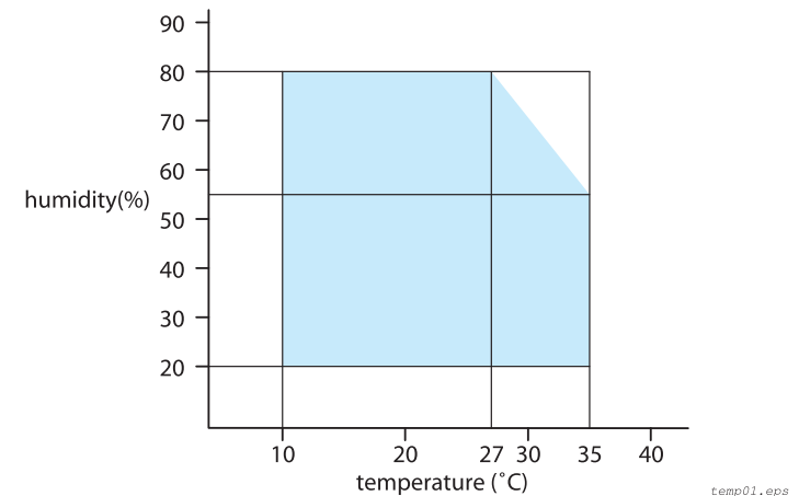
Figure 1-6. Temperature/Humidity Range
