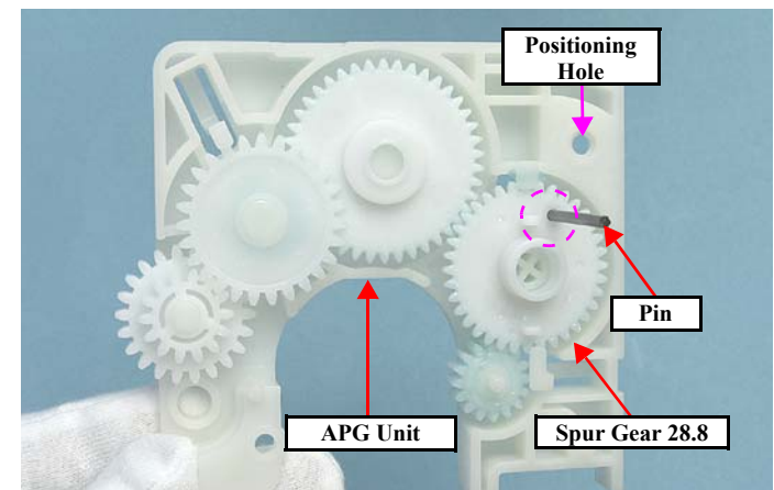
Figure 4-92. Reinstalling the APG Unit (2)
