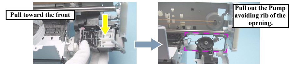
Figure 4-118. Removing the Ink System (2)
