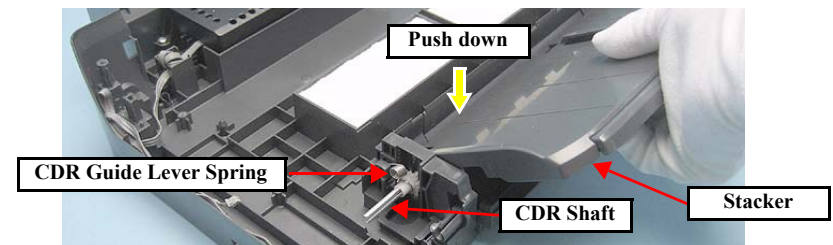
Figure 4-109. Removing the CDR Guide Lever Spring (1)
