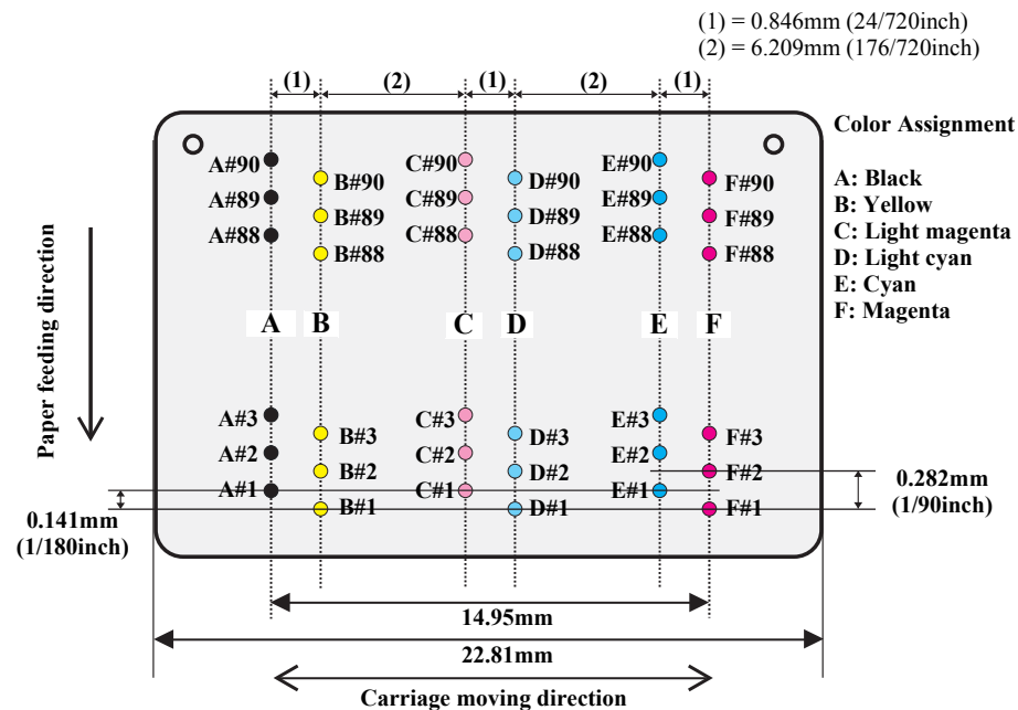
Figure 1-2. Nozzle Configuration
