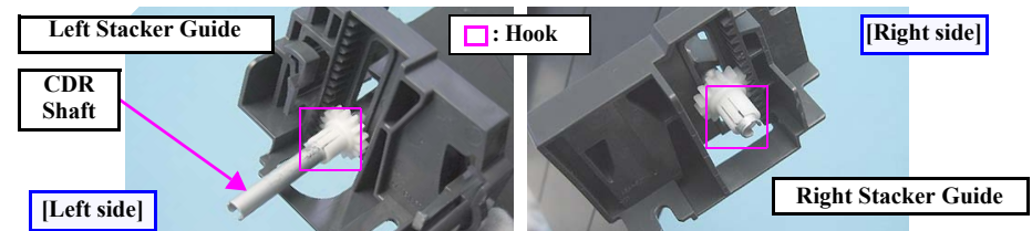
Figure 4-112. Removing the CDR Shaft
