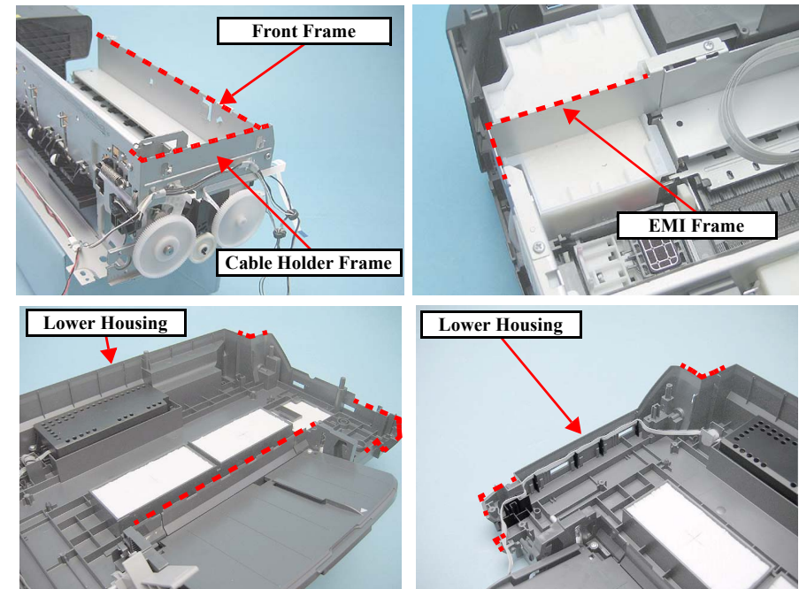
Figure 4-9. Sharp Metal Edges
