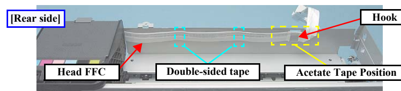
Figure 4-127. Removing the Head FFC
