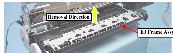
Figure 4-130. Removing the EJ Frame Assy
