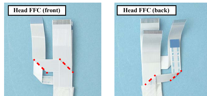
Figure 4-50. Routing the Head FFC (2)
