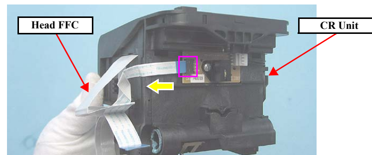
Figure 4-150. Removing the CR Unit (6)
