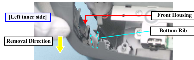
Figure 4-38. Caution as to Removing the Front Housing
