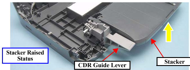
Figure 4-83. Cautions on Removing the Printer Mechanism
