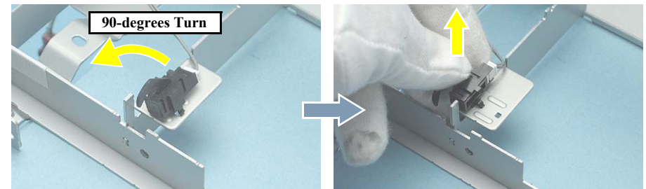
Figure 4-165. Removing the CDR Tray Sensor (CDR Guide Detection Assy)
