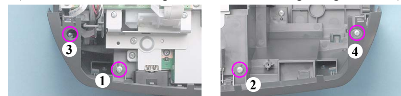
Figure 4-36. Removing the Front Housing (1)
