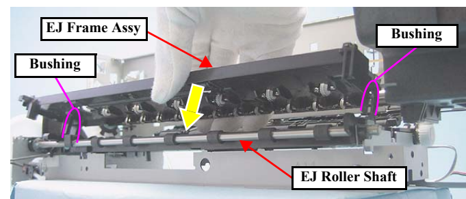
Figure 4-131. Reinstalling the EJ Frame Assy
